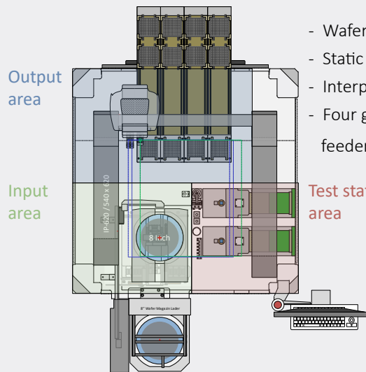
KGD Test Handler 8" Wafer
